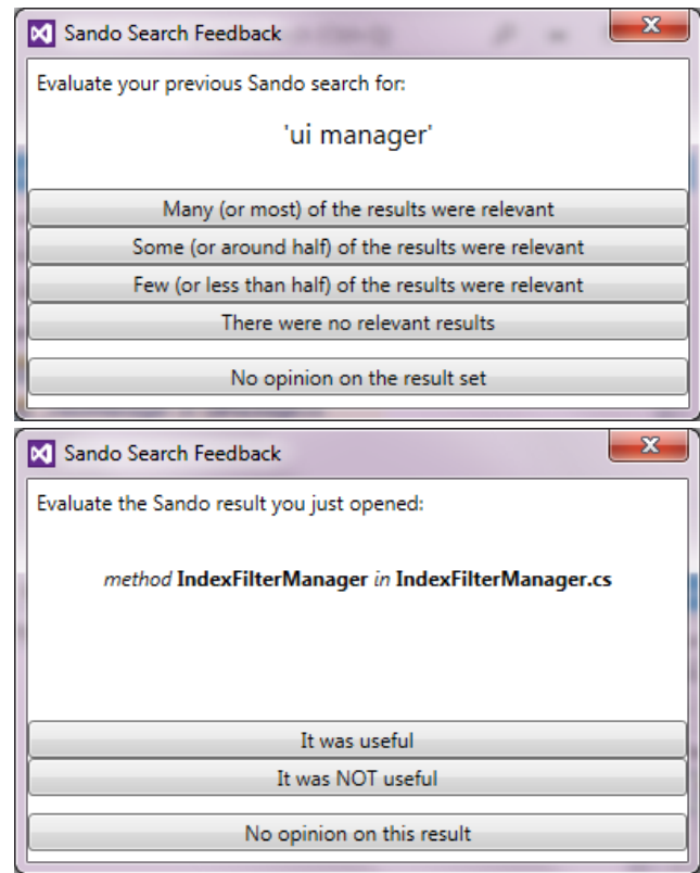
Fig. 1. Popups to gather participant feedback for entire result set (top), and a clicked result (bottom).
