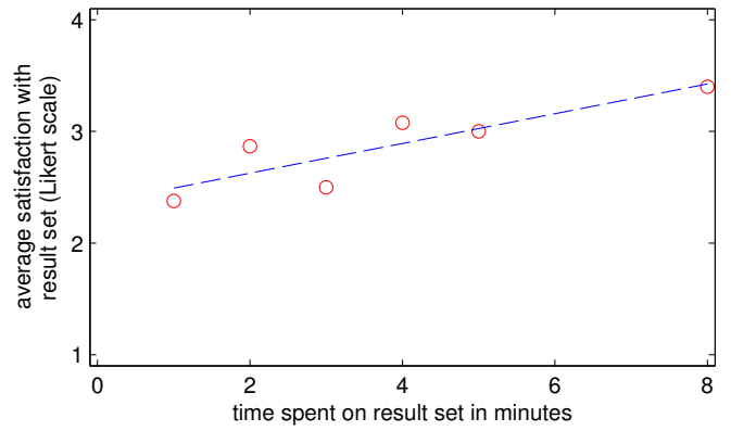
Fig. 3. Exploratory Study: A plot of developer usage metrics, NUMBER OF CLICKS (left) and TIME ON RESULT SET (right), to user satisfaction represented by a Likert scale of 1-4. Each plot includes data points representing average satisfaction for a specific metric value with at least 5 data points and a regression line.
