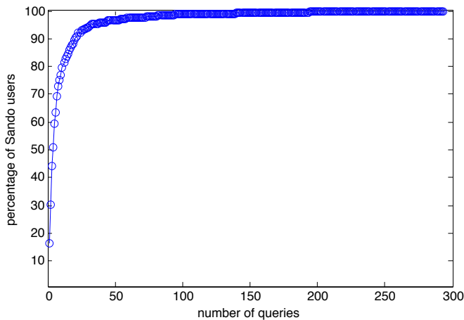
Fig. 4. Cumulative distribution function of the percentage of Sando users issuing a certain number of queries.
